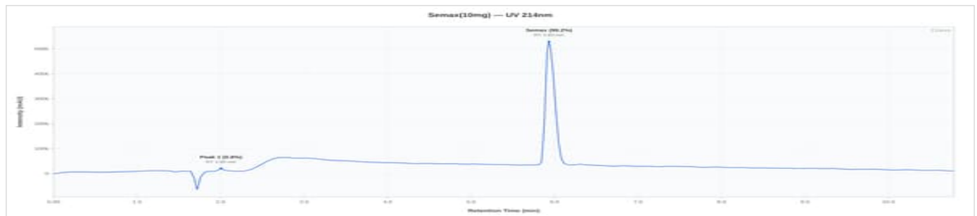
Semax 10mg - 001-R: UV Chromatogram
